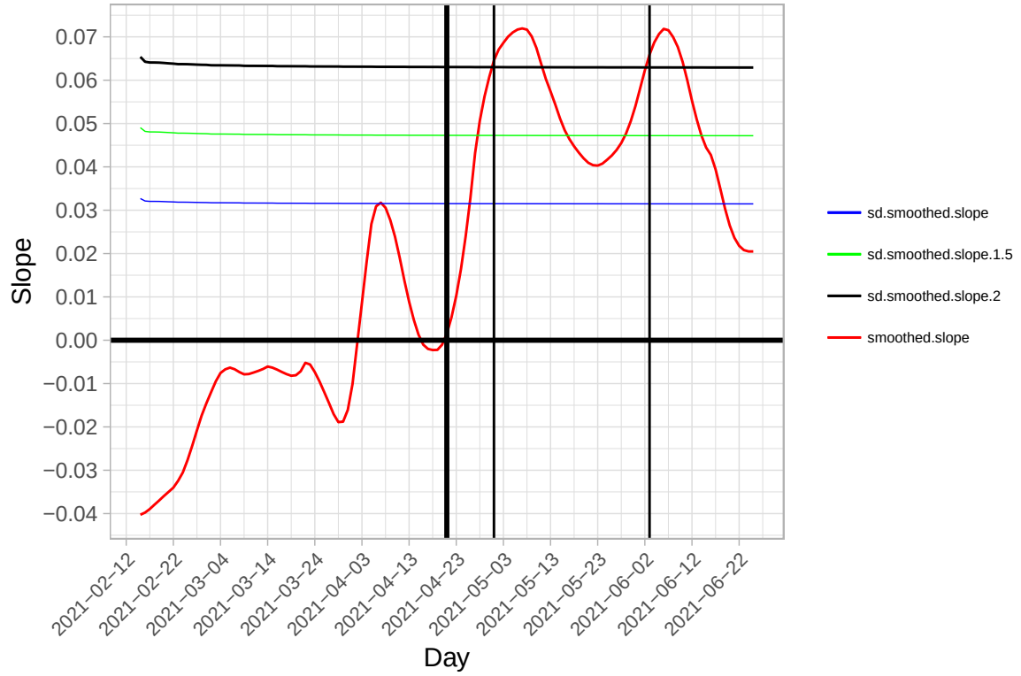
Figure 6: Reinitialisation rule for the sample ending on 25 June 2021. The endpoint trigger is satisfied when \hat{\gamma}_{T|T} exceeds zero by two standard errors. The reset date supplied to reinit.date is then backdated to 21 April 2021, the start of the current positive spell in the smoothed slope estimate computed on that same sample.
