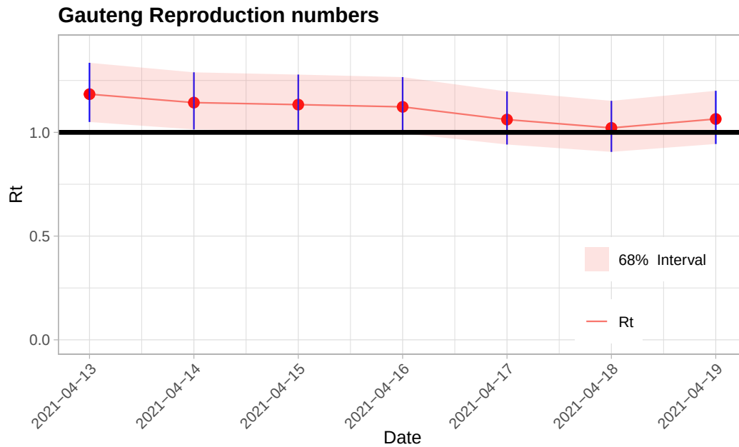
Figure 5: Model-implied reproduction numbers for the 7-day period to 19 April 2021 for Gauteng province in South Africa. Bands are approximate pointwise uncertainty bands conditional on a four-day generation interval.
