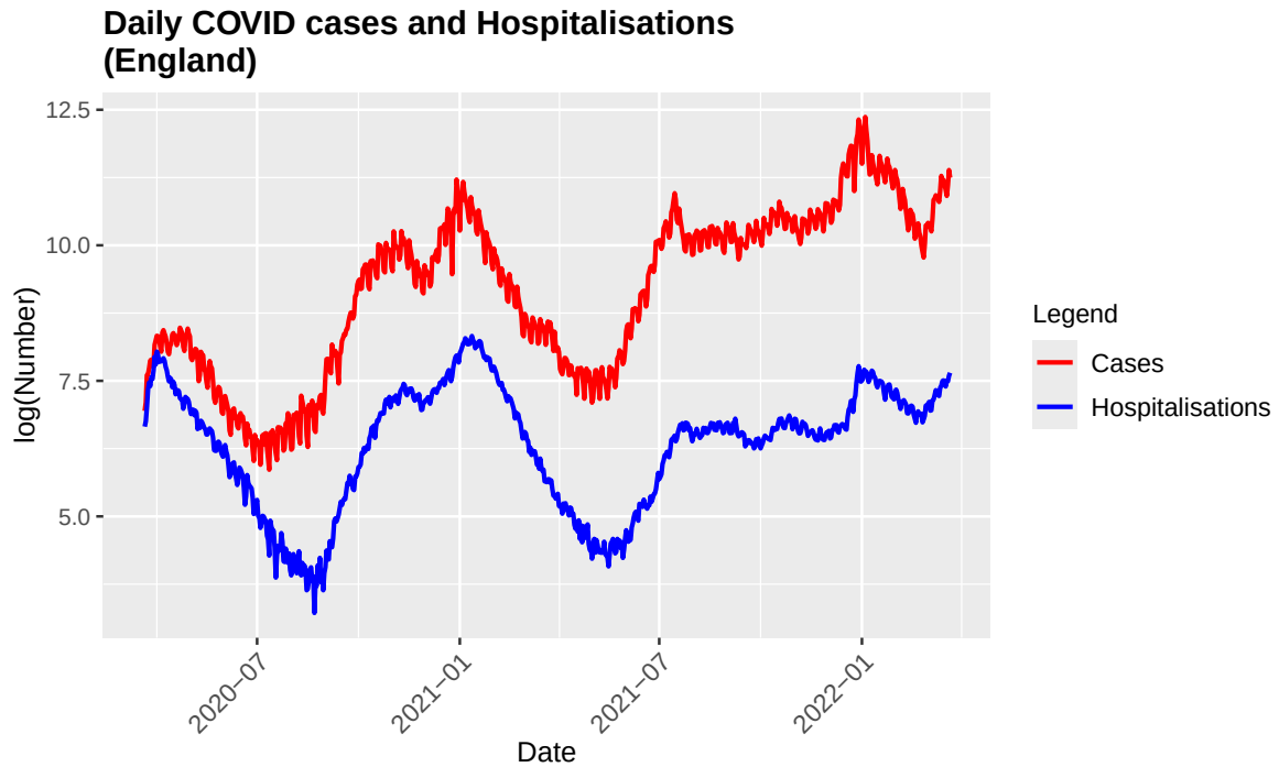
Figure 10: England daily cases and hospitalisations.
