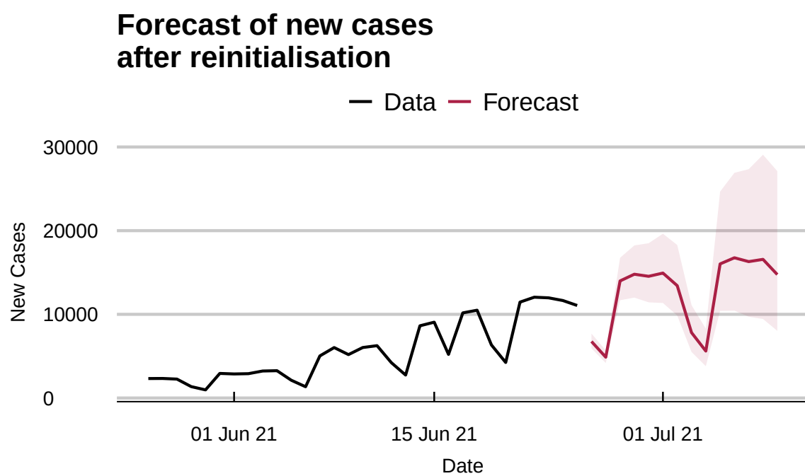
Figure 8: Forecast of new cases after reinitialisation. The shaded region is a state-implied forecast band.
