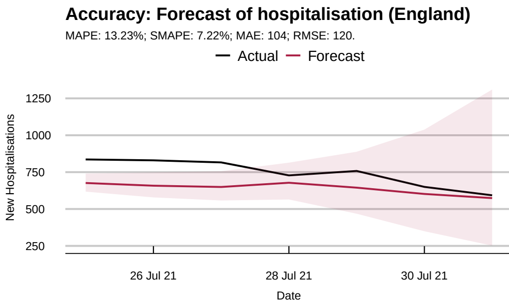
Figure 11: Accuracy of the seven-day forecast of hospitalisations for England.
