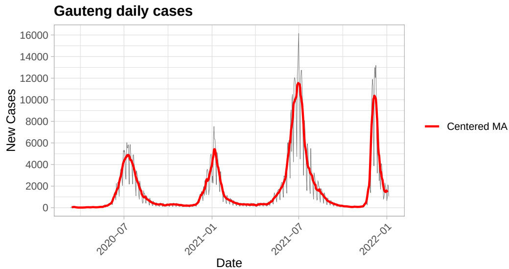
Figure 1: New cases and their centered 7-day moving average for Gauteng province in South Africa between 10 March 2020 and 5 January 2022.
