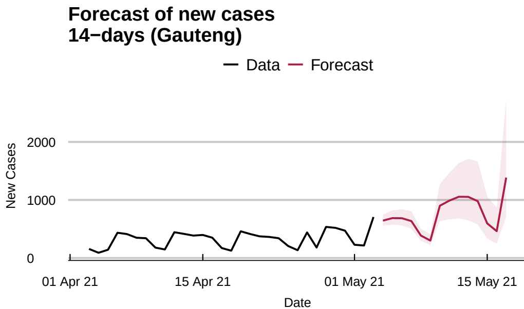
Figure 3: Fourteen-day forecast of new cases from 4 May 2021 for Gauteng province in South Africa. The shaded region is a state-implied forecast band obtained by propagating uncertainty in the latent log growth rate.
