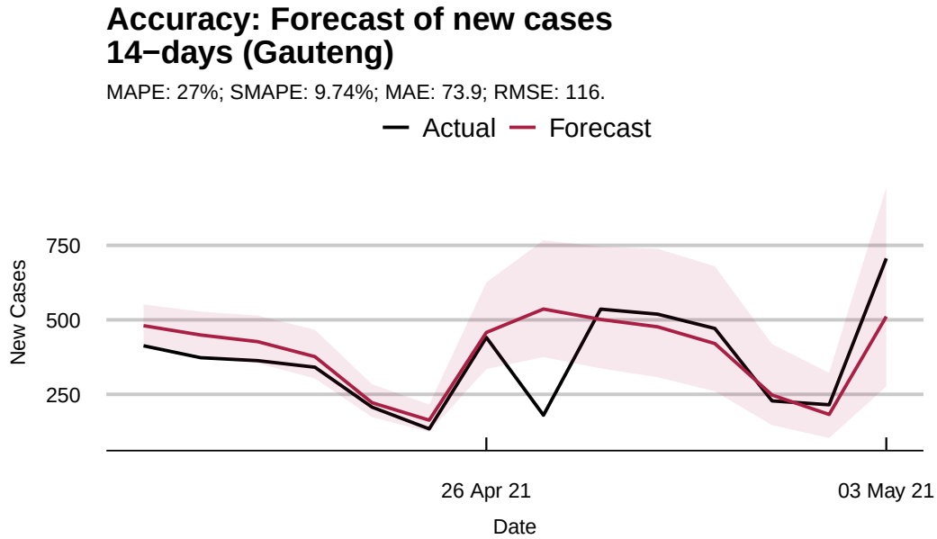
Figure 4: Accuracy of the fourteen-day forecast of new cases from 20 April 2021 for Gauteng province in South Africa.
