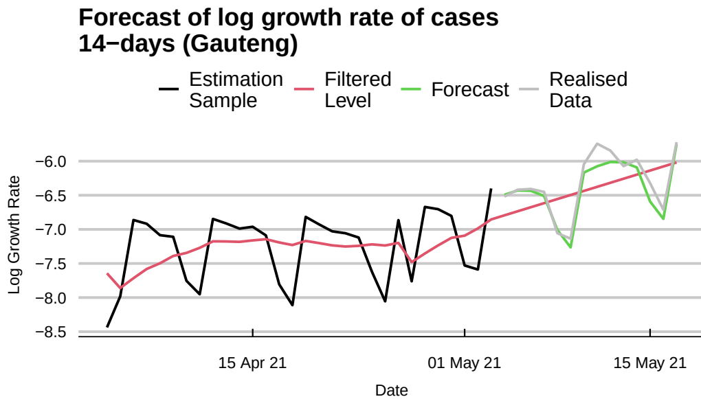
Figure 2: Fourteen-day forecast of \ln(g_t) from 4 May 2021 for Gauteng province in South Africa.
